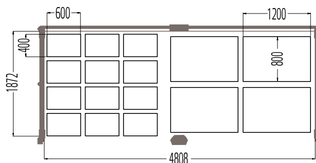
Sample plan of practical option for filling with pallets (bird's eye view)
