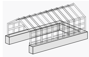
Strip foundations, U-shaped
