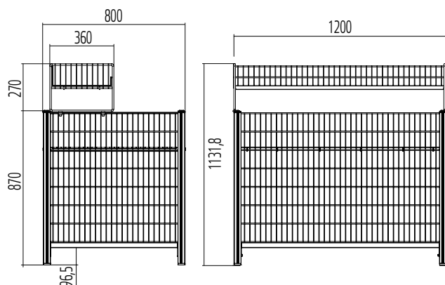
Stationary FlexTable Basic with table-top attachment
