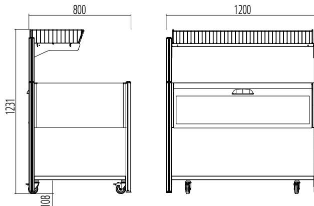
FlexTable Premium with table-top attachment, mobile
